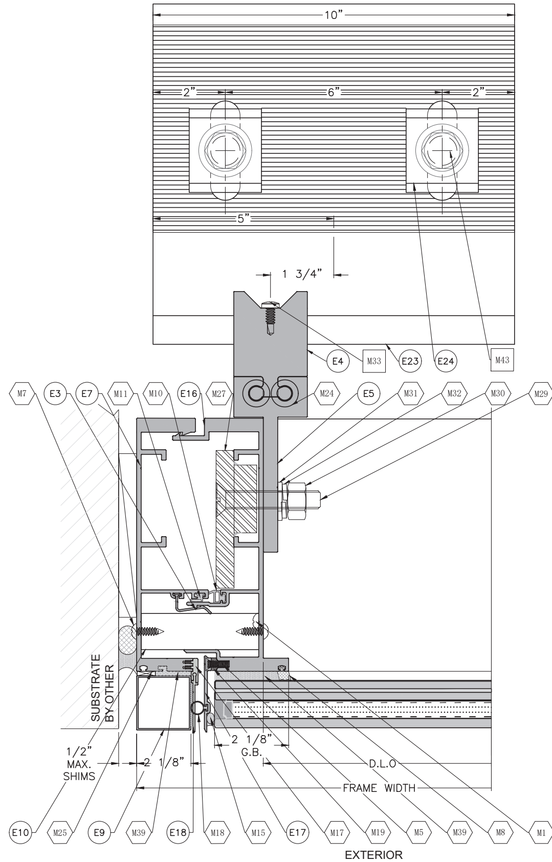
1 D5 DETAIL
