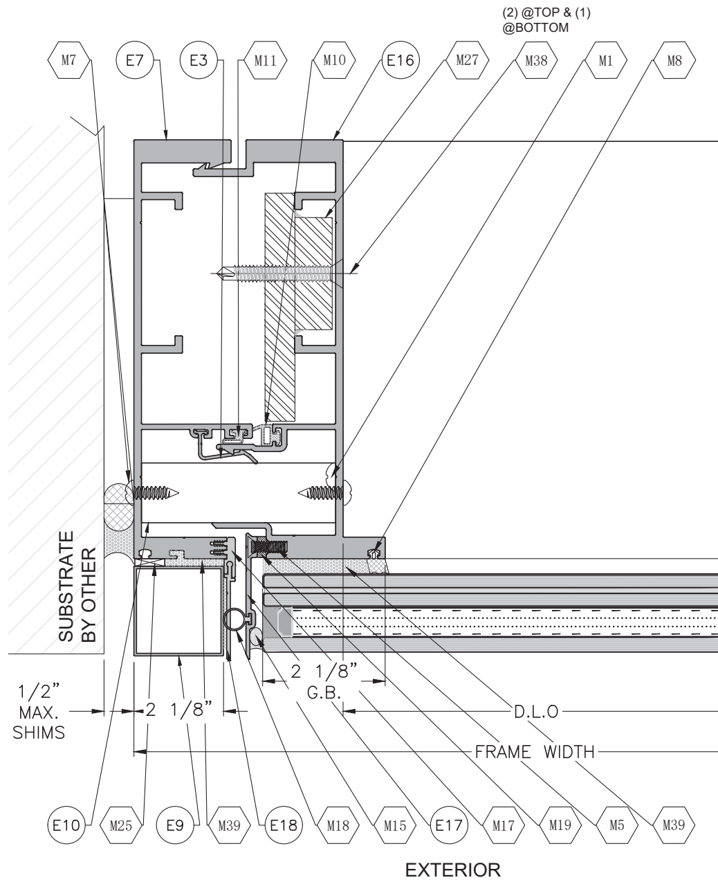
1 D3 DETAIL
